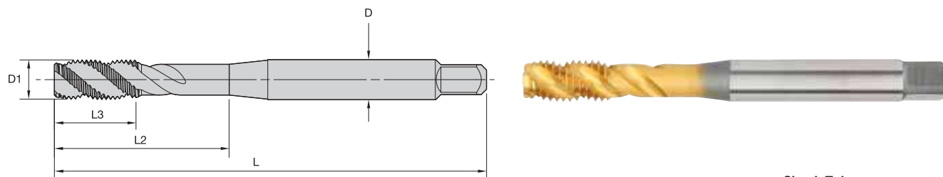
Shank Tolerance
