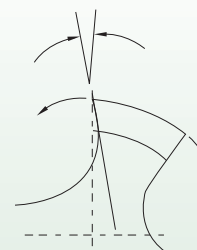
Positive Rake
